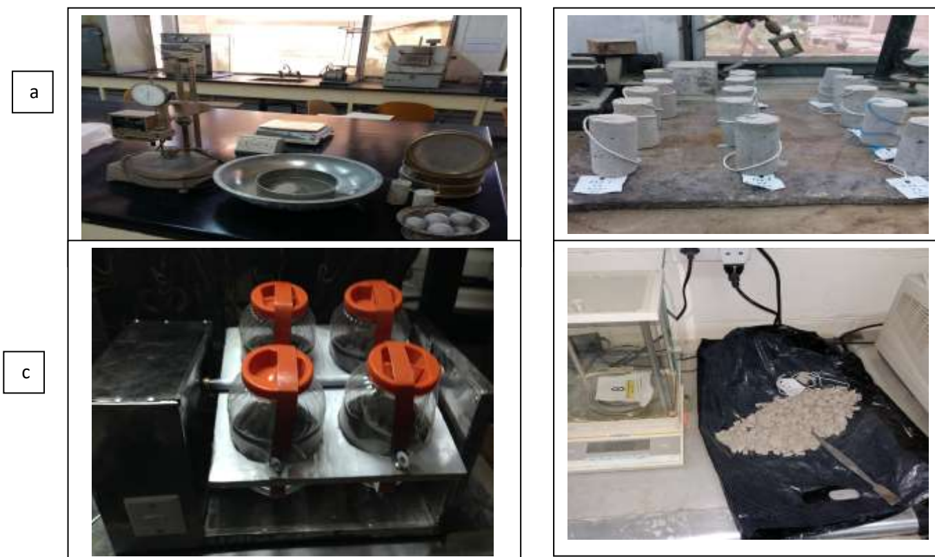
Fig 2. Experimental apparatus and the S/S specimens
